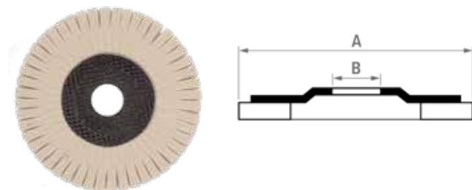
Type FG 27 (flat) reduced backing
